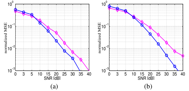
Fig. 2: Normalized MSE vs. SNR obtained with matrix modulation using the iterative demodulation algorithm. (a) One data stream, M_T = 2 ( \diamond ) or M_T = 4 ( \circ ) transmit antennas, and M_R = 2 receive antennas; (b) three data streams assigned to a single user ( \diamond ) or to three different users ( \circ ).
