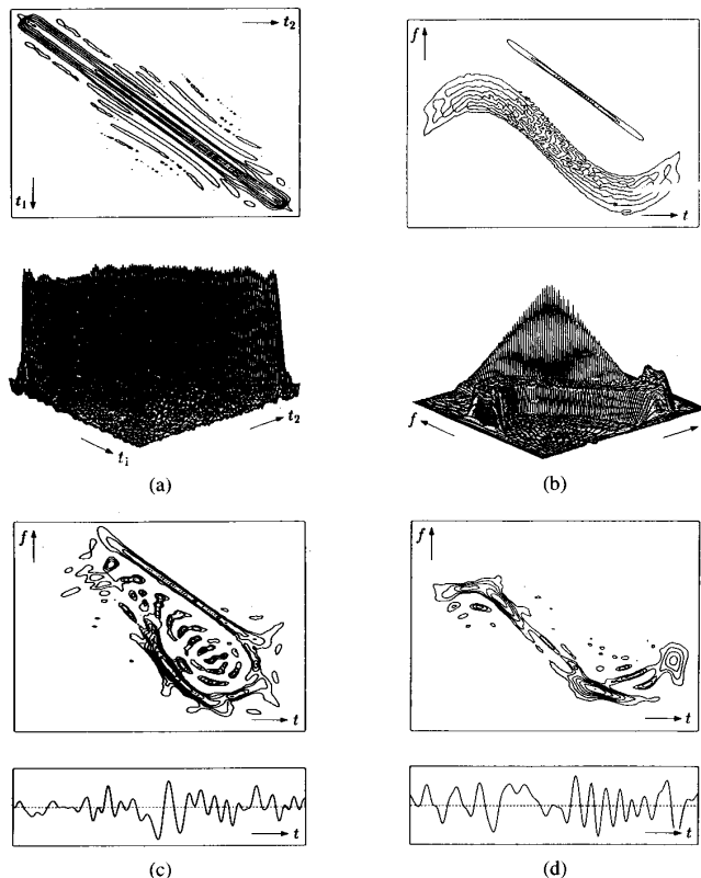
Fig. 1. Comparison of the ACF and the WVS for a nonstationary process consisting of two statistically orthogonal components. (a) Magnitude of ACF, (b) WVS, (c) and (d) real parts and Wigner distributions (incorporating a small amount of TF smoothing) 2 of two realizations of the process.
