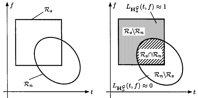
Fig. 2. TF interpretation of the time-varying Wiener filter.
