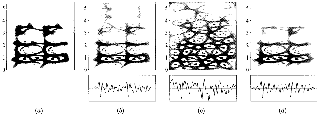
Fig. 8. Speech enhancement experiment using TF pseudo-Wiener filter. (a) WS of TF pseudo-Wiener filter \mathbf{H}_1 . (b) Two pitch periods of noise-free speech signal. (c) Noise-corrupted speech signal. (d) Enhanced speech signal. All signals are represented by their time-domain waveforms and their (slightly smoothed) Wigner distributions [19], [58], [60], [61]. Horizontal axis: time (signal duration is 256 signal samples, corresponding to 2.32 ms). Vertical axis: frequency in kilohertz.
