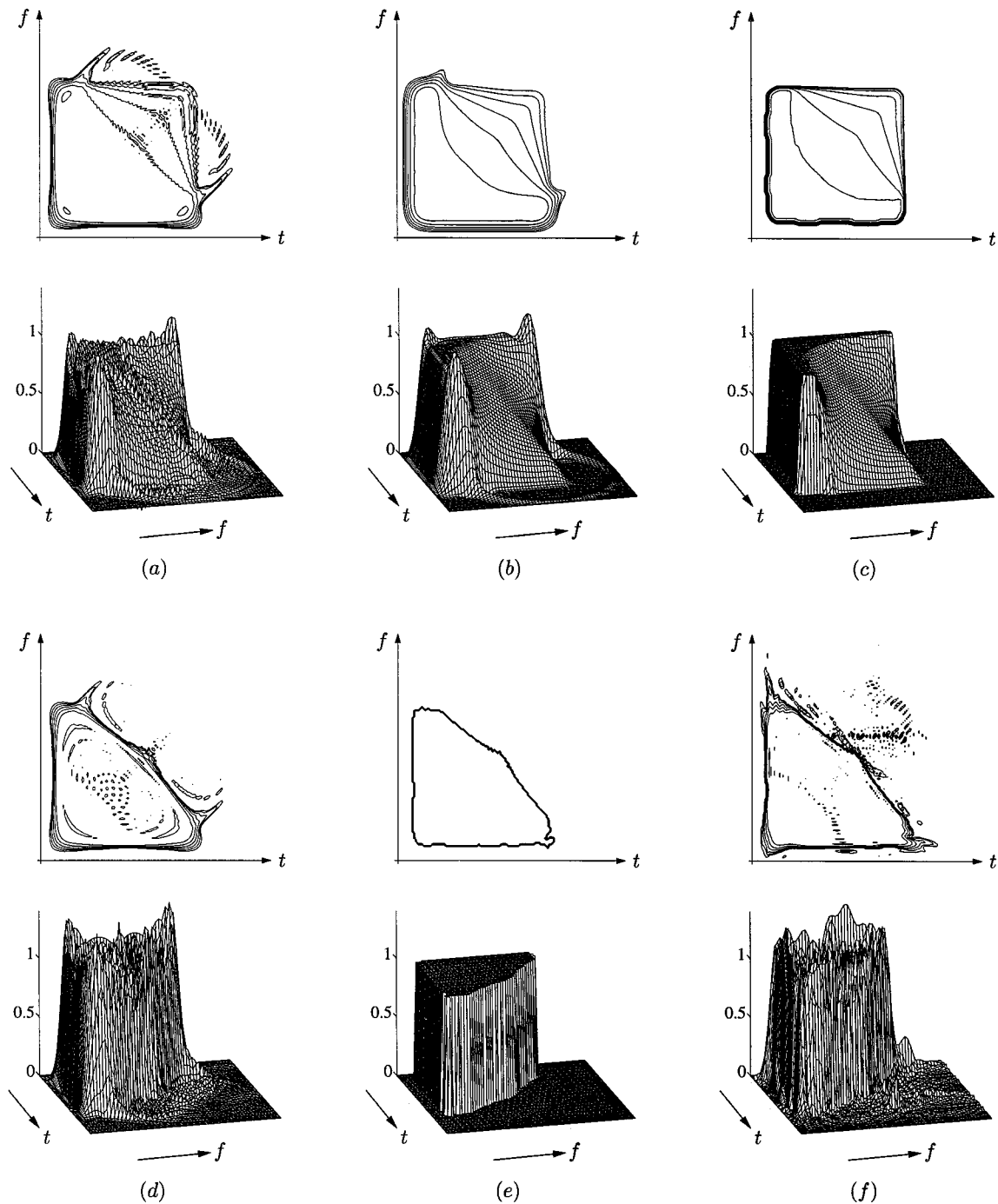
Fig. 5. WS's of (a) Wiener filter \mathbf{H}_o . (b) Underspread part \mathbf{H}_o^u of Wiener filter. (c) TF pseudo-Wiener filter \mathbf{H}_1 . (d) Optimal projection filter \mathbf{P}_o . (e) TF pseudo-projection filter \mathbf{P} . (f) TF projection filter \mathbf{P}_1 .
