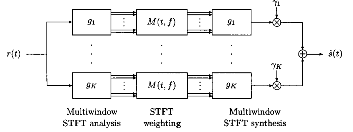
Fig. 3. Multiwindow STFT implementation of the Wiener filter.
