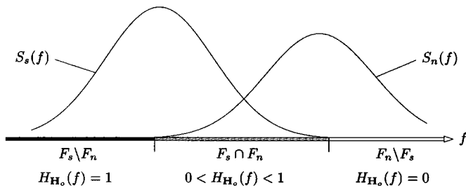
Fig. 1. Frequency-domain interpretation of the time-invariant Wiener filter.
