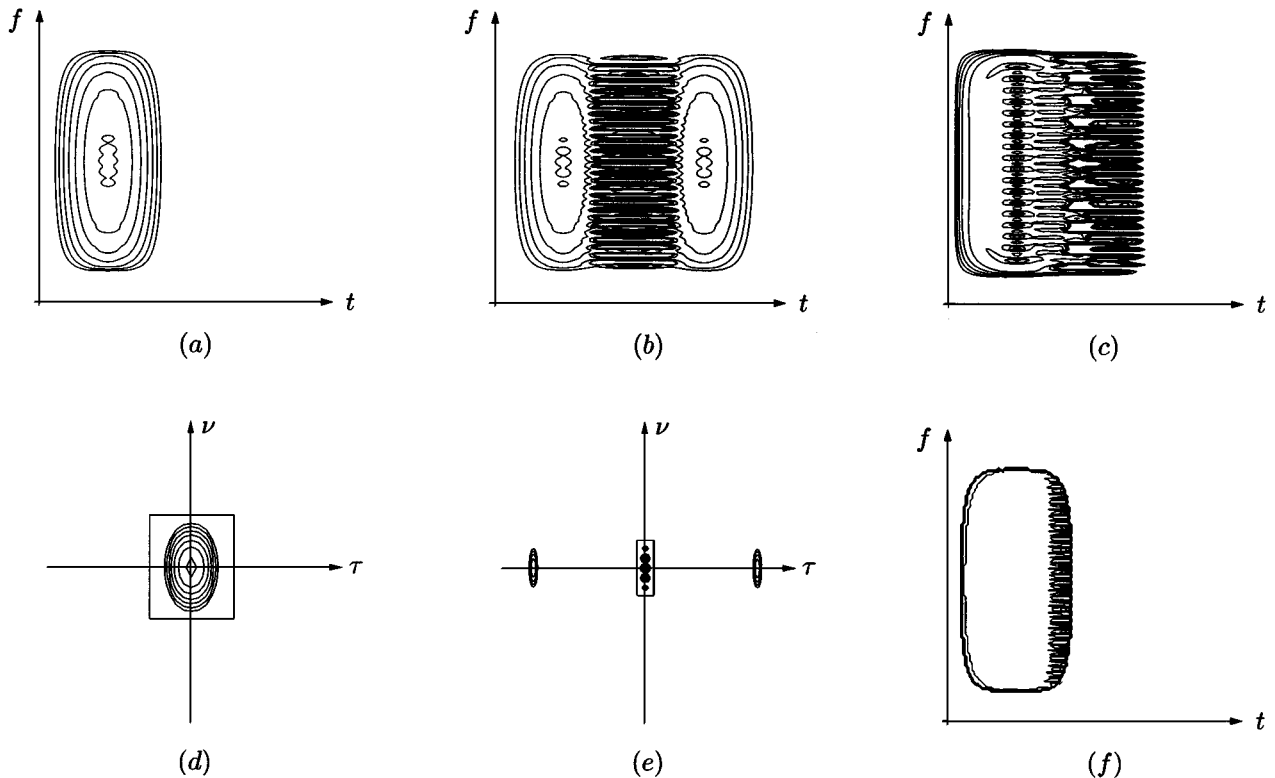
Fig. 7. Filtering experiment involving an overspread noise process. (a) WVS of s(t) . (b) WVS of n(t) . (c) WS of Wiener filter \mathbf{H}_o . (d) Expected ambiguity function of s(t) . (e) Expected ambiguity function of n(t) . (f) WS of TF pseudo-Wiener filter \mathbf{H}_1 . The rectangles in parts (d) and (e) have area 1 and thus allow assessment of the under-/overspread property of s(t) and n(t) . (In particular, part (e) shows that n(t) is overspread.) The signal length is 128 samples.
