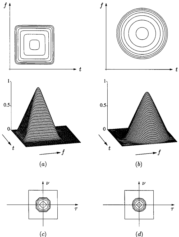
Fig. 4. Second-order statistics of signal and noise. (a) WVS of s(t) . (b) WVS of n(t) . (c) Expected ambiguity function of s(t) . (d) Expected ambiguity function of n(t) . The rectangles in parts (c) and (d) have area 1 and thus allow assessment of the underspread property of s(t) and n(t) . The signal length is 128 samples.
