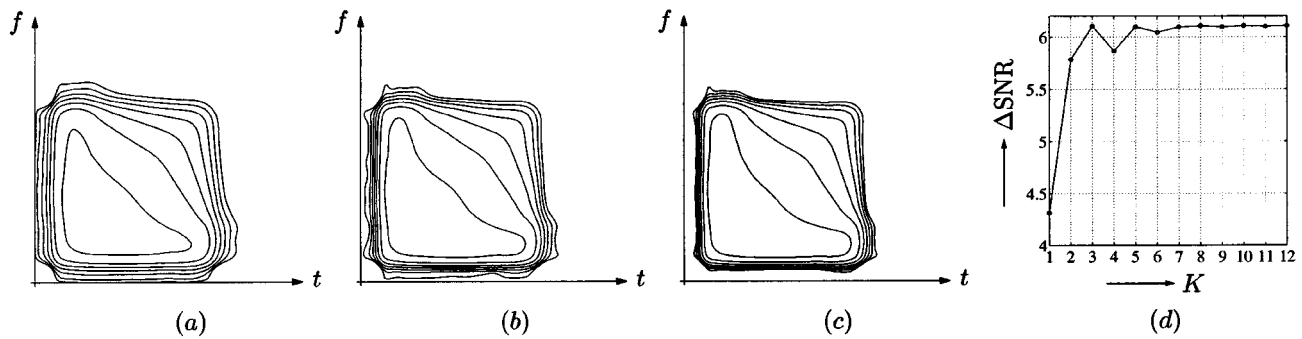
Fig. 6. Multiwindow STFT implementation of the Wiener filter. (a)–(c) WS's of multiwindow STFT filters with filter order K = 1, 4 , and 10 . (d) Mean SNR improvement versus STFT filter order K .
