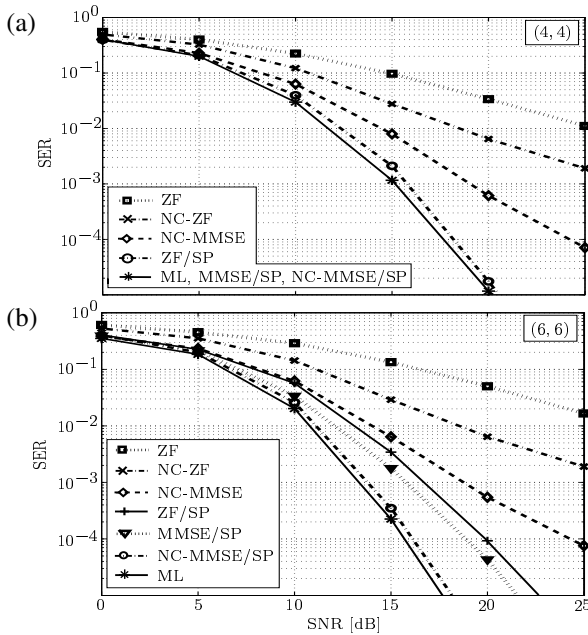
Fig. 4. SER vs. SNR performance of various SPA and standard detectors using 4-QAM modulation: (a) (4, 4) system, (b) (6, 6) system.
