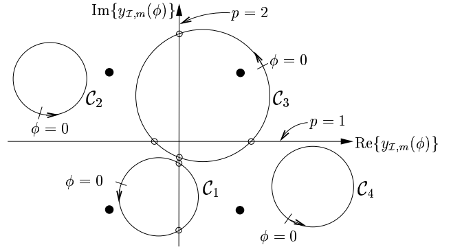
Fig. 3. Component circles \mathcal{C}_m for a (4, 4) channel and 4-QAM modulation ( P = 2 ). (All 4 component circles are drawn in a common complex plane.) When moving along the intersection circle \mathcal{I} (by varying \phi ), the m th component y_{\mathcal{I},m}(\phi) of \mathbf{y}_{\mathcal{I}}(\phi) moves along the component circle \mathcal{C}_m .
